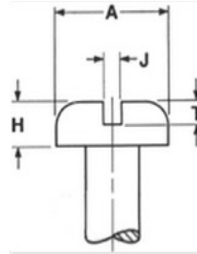
Slotted Drive
